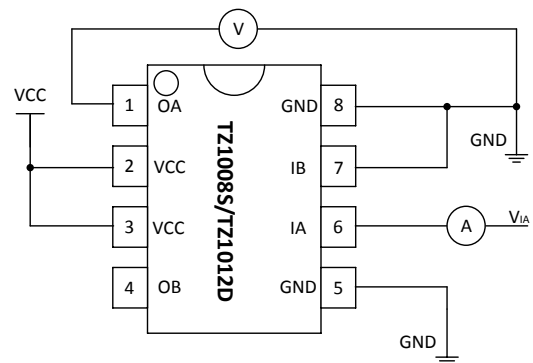
Fig. 2 (Input current I_{IN} )
